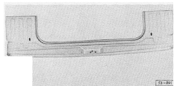
Fig. 10: Preparing rear floor plate (new part)
