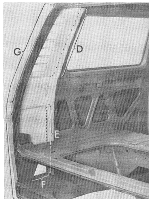
Fig. 13: Welding in corner panel and gusset plate
