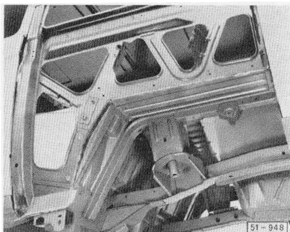
Fig. 3: Inner wheel housing
