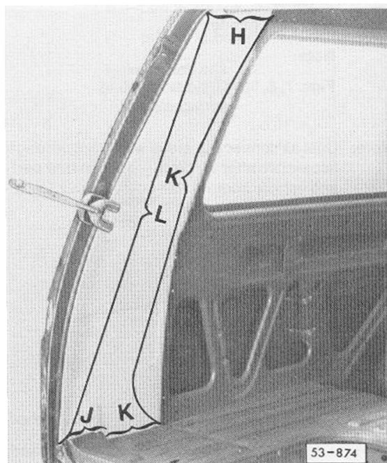
Fig. 15: Corner panel
