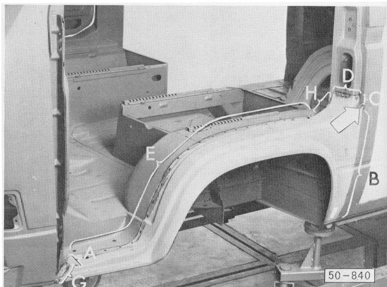
Fig. 6: Aligning and welding in wheel arch panel
