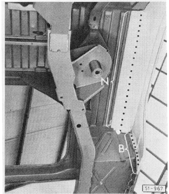
Fig. 11: Welding in inner wheel housing
