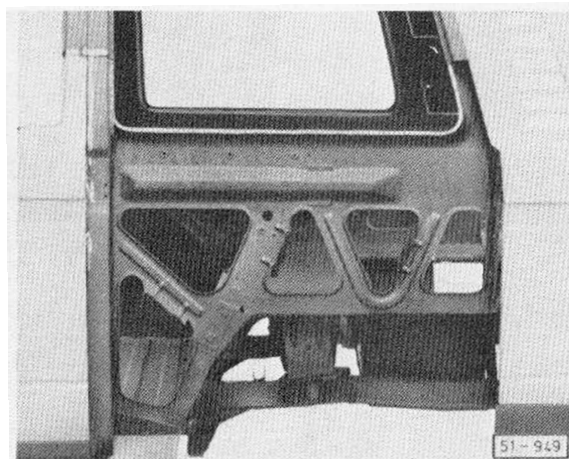
Fig. 4: Inner wheel housing and outer side panel
